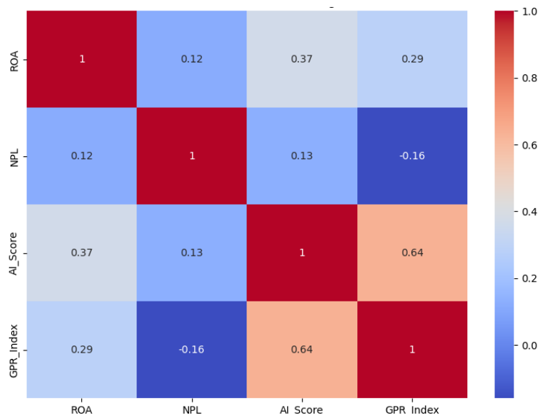
Figure 1. Heatmap Correlation Source: Data Processed, Phyton (2025)
