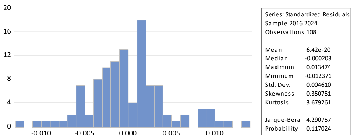
Figure 1. Normality Test
