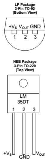
Gambar 3. Konfigurasi Pin LM-35. (Sumber : Texas Instruments, 2017)
