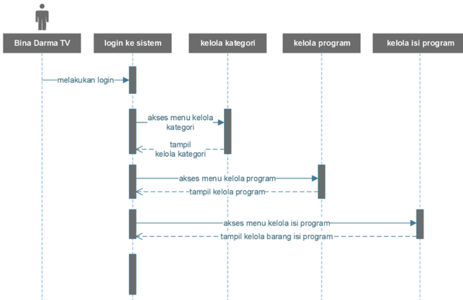
Gambar 4. Sequence Diagram Bina Darma TV (Administrator)
