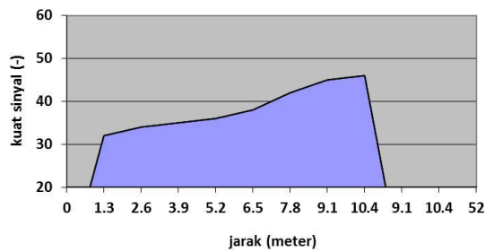
Figure 8. Relationship graph between distance and access point signal strength with mac address OC:85:25:F3:A8:D4 on 4 th floor
