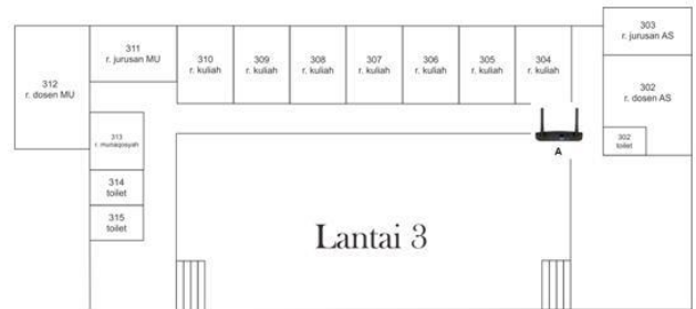
Figure 11. Good access point installment position on 3 rd floor
