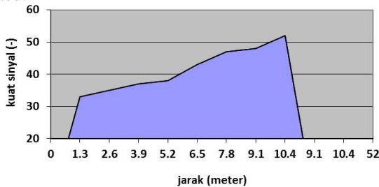
Figure 7. Relationship graph between distance and access point signal strength with mac address OC:85:25:F3:5C:D4 on 3 rd floor
