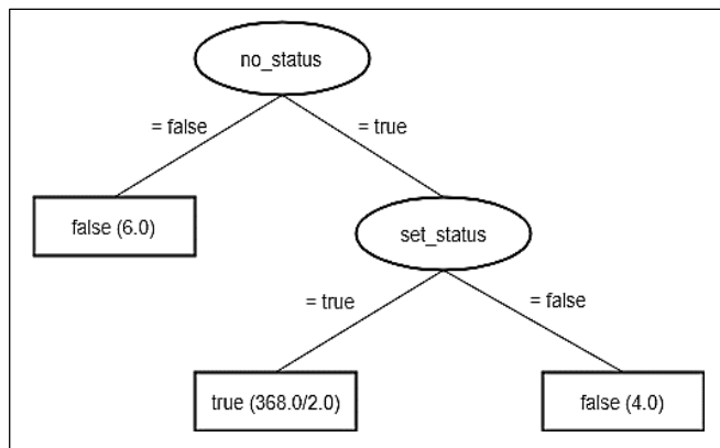
Figure 5. Decision Tree using Supplied Data Test
