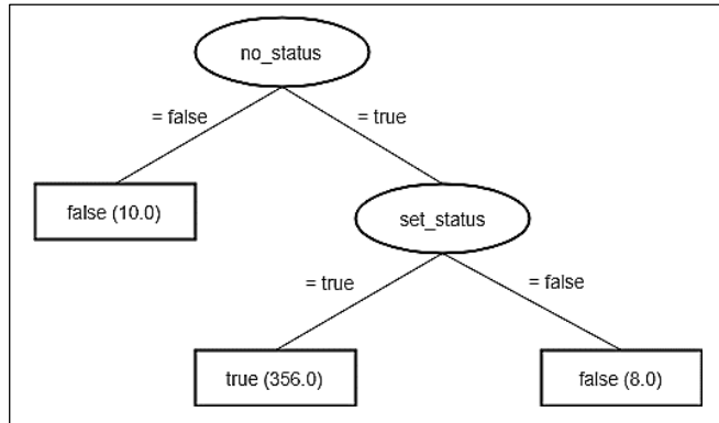
Figure 4. Generated Decision Tree
