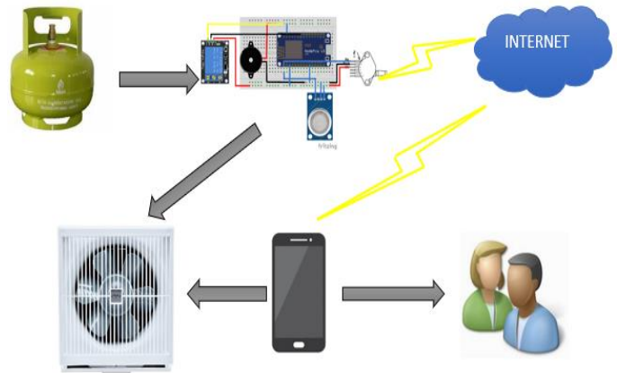
Figure 1. Architecture of a Gas Leak Detection System
