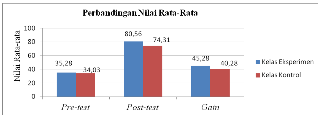
Diagram 1. Perbandingan nilai rata-rata pre-test , post-test dan gain
