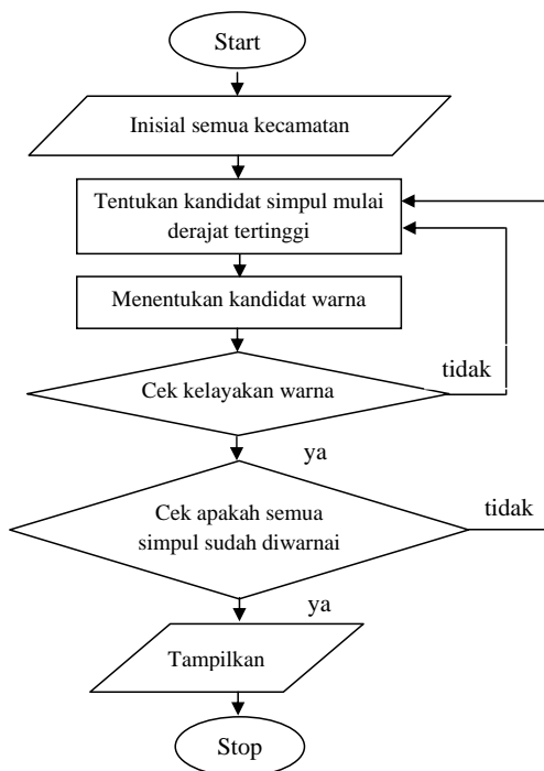
Gambar 5. Flowchart Algoritma Greedy Coloring
