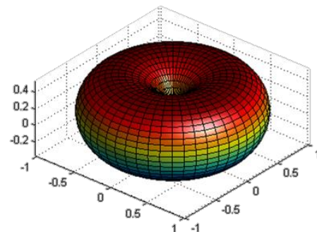
Figure 3. Interrupted Angular Wave Function \nu = \mu = 1 untuk n_l = 0, m = 0 .
