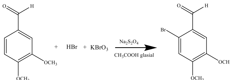
Figure 1. Synthesis 6-bromoveratraldehyde
