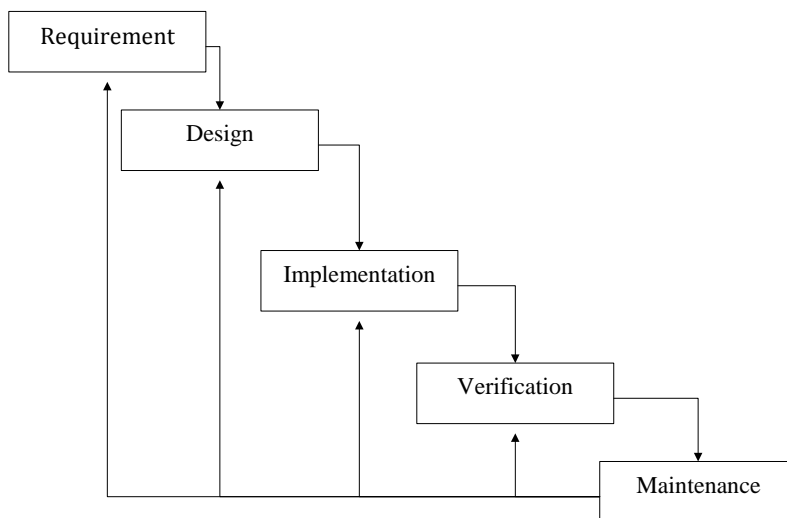
Chart 1. Waterfall Model
