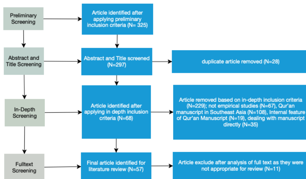
Figure 1. PRISMA flowchart
